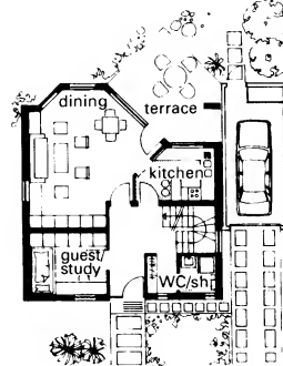
12 House with rooms in roof space
